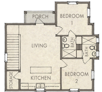
OPTIONAL CARRIAGE HOUSE
