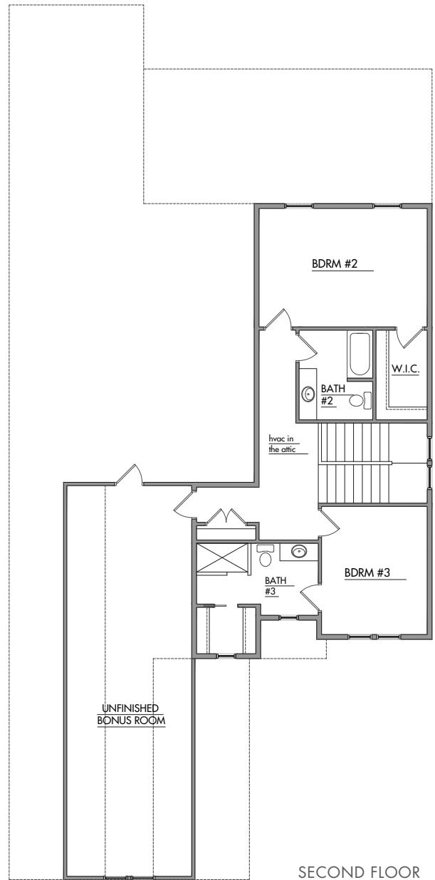
SECOND FLOOR
