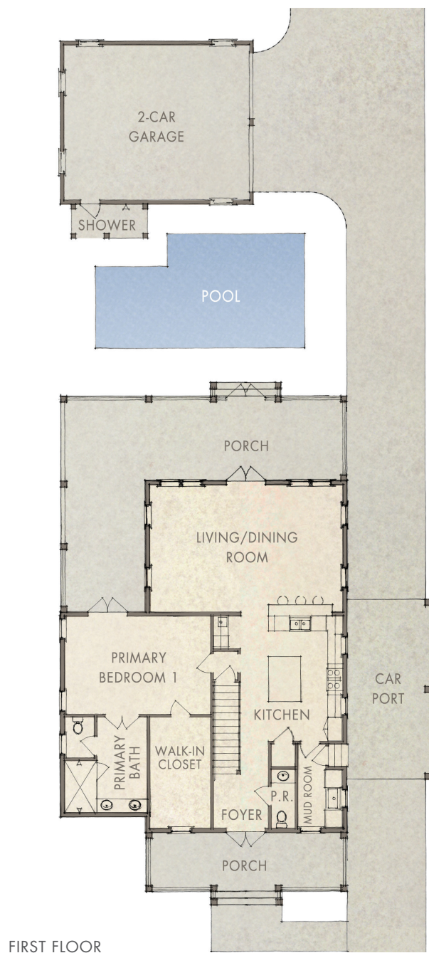
FIRST FLOOR
